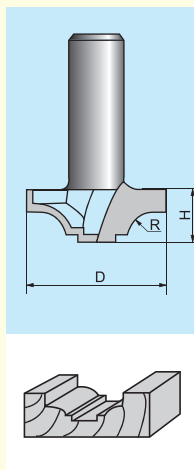
0705 CLASSICAL BIT 台階圓弧刀
