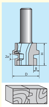
1609 MITER BIT 斜齒樺刀
