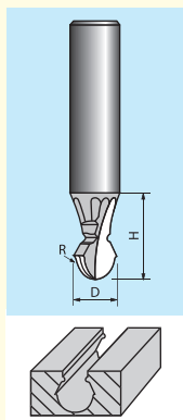
1611B KEYHOLE BIT 門板拉直刀(三刃)
