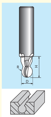
1611A KEYHOLE BIT 門板拉直刀(三刃)
