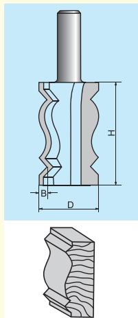
1010 CROWN MOULDING BIT 流線扶手刀
