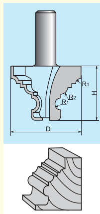
1011 PALACE TYPE BIT 花線刀
